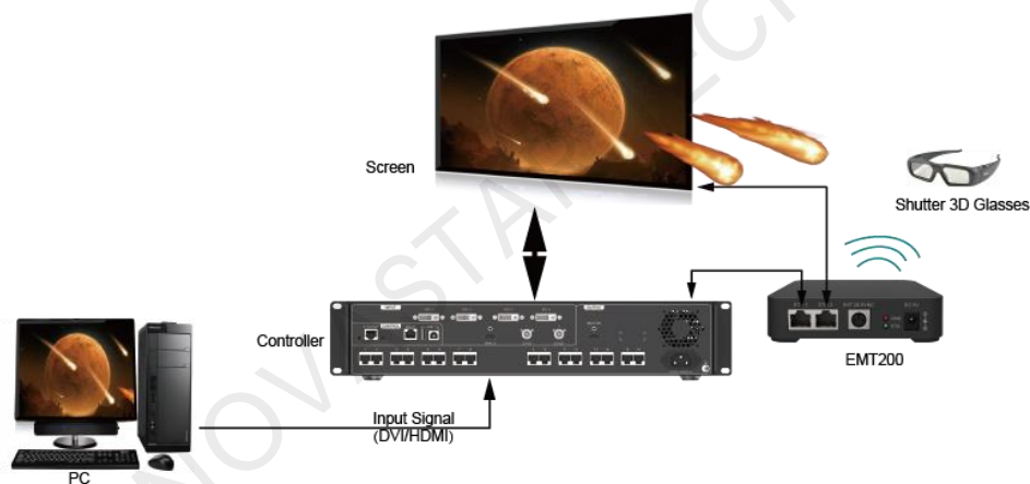
Figure 5-19 Hardware connections
